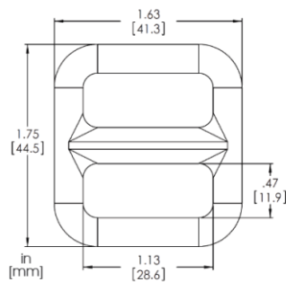
buckle dimensions
