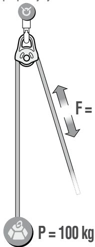
6A. Simple pulley system
